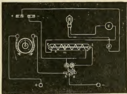
FIG. 115. — Diagram of switch board for regulating lighting currents by means of shunt.
